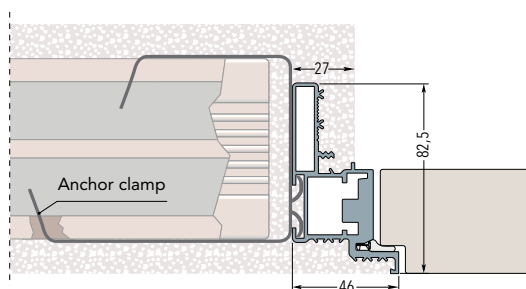
Frame on solid wall
