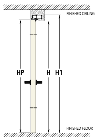
FRAME WITH HEADER
