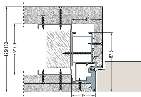
Frame on stud wall with two layer of plasterboard - Finished wall thickness 125/150 mm
